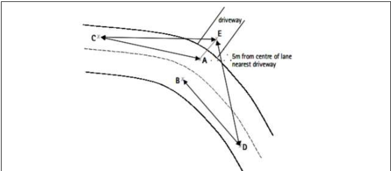
Figure 18: Lines of clear sight measurements from RTS6
